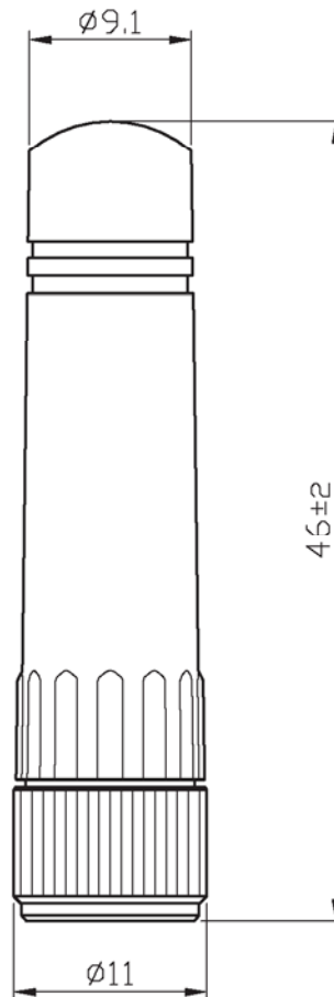
Reverse SMA Plug
