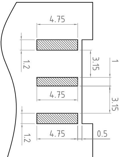
Recommended PCB Soldering Pattern
